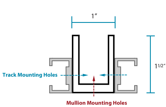
"H" Mullion
